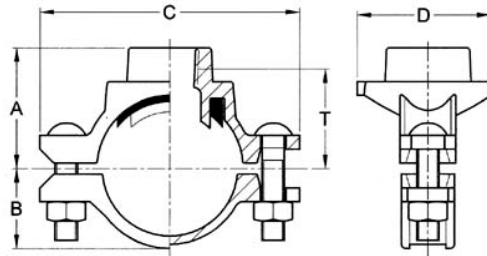
Model SS-723 Stainless Steel Mechanical Tee
